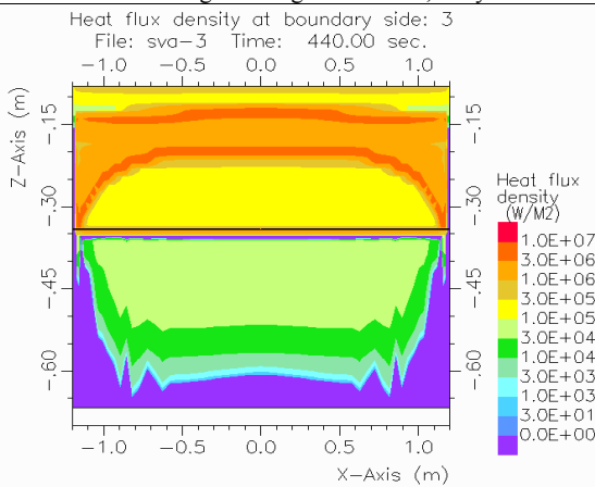
Figure 4b. Heat flux, 610x2400 mm model ingot rolling side at 440 s, alloy 5083
