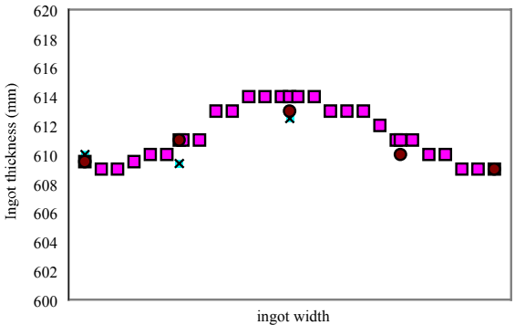
Figure 13. 610x2700 mm ingot thickness at steady state
