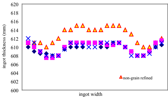
Figure 12. 610x2400 mm ingot thicknesses at steady state
