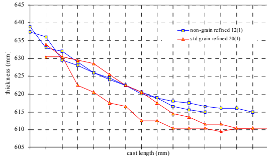
Figure 16. Thickness over length (e.g. swell) 610x2400 mm
