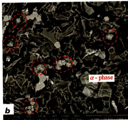
Fig 3. SEM image showing the morphology of intermetallic compounds present in: (a) non-US sample treat; (b) US sample treated
