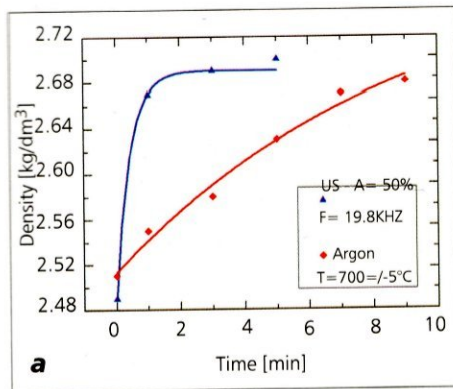
Fig 2. (a) Density of the AlSi9Cu3 alloy as a function of ultrasonic degassing time; (b) porosity in sample before US degassing; (c) porosity in sample after 3 of US degassing
